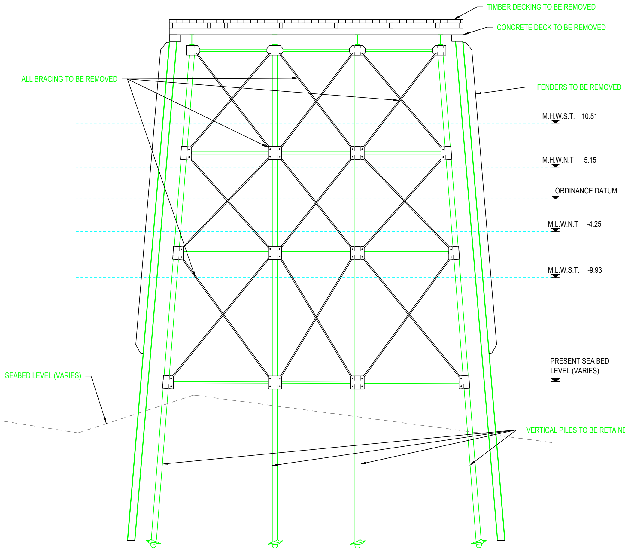
JETTY CROSS SECTION - EXISTING
