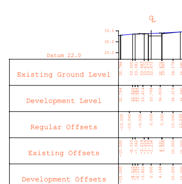
Cross Section number 36 ( 192170.3E 204926.3N ) Cross Section number 41 ( 192220.0E 204931.0N ) Cross Section number 46 ( 192258.3E 204961.3N ) Cross Section number 51 ( 192292.9E 204997.3N ) Cross Section number 56 ( 192327.7E 205033.3N ) Cross Section number 61 ( 192361.9E 205069.6N )
