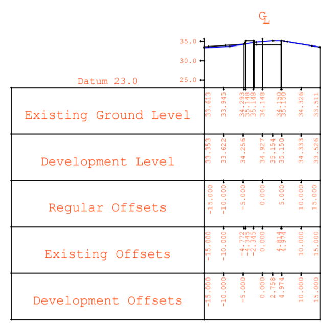
Cross Section number 34 ( 192150.5E 204929.1N ) Cross Section number 39 ( 192200.2E 204927.9N ) Cross Section number 44 ( 192244.5E 204946.8N ) Cross Section number 49 ( 192279.1E 204982.9N ) Cross Section number 54 ( 192313.7E 205018.9N ) Cross Section number 59 ( 192347.9E 205055.4N ) Cross Section number 64 ( 192385.5E 205088.1N )
