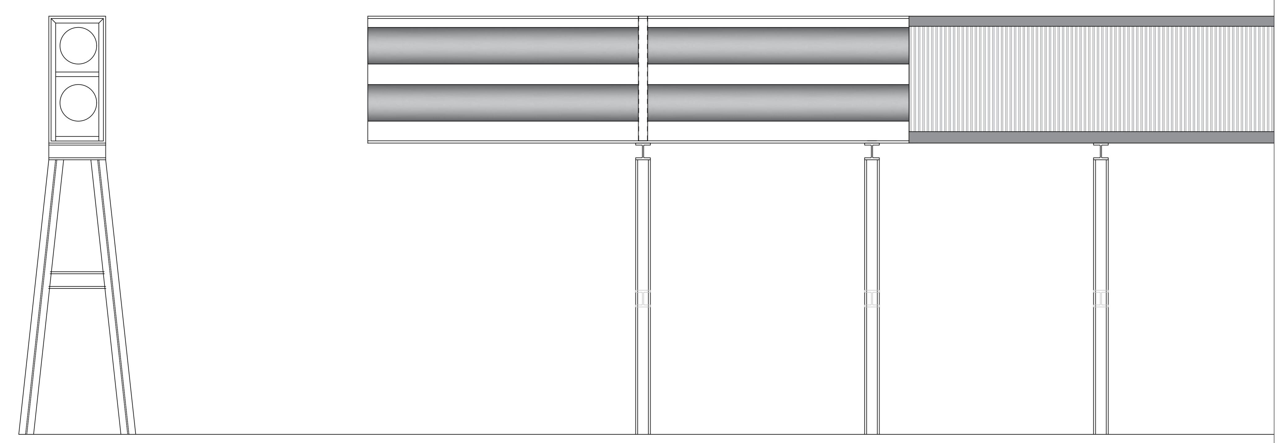
TYPICAL CONVEYOR CROSS SECTION - TYPE 3 SCALE 1:50
